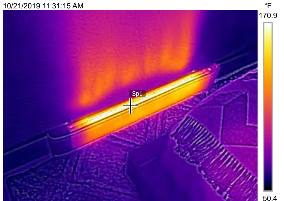
ELECTRIC BASEBOAR...
